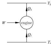
Fig. 13.9 A refrigerator or a heat pump. Both devices are heat engines run in reverse (i.e. reversing the arrows on the cycle shown in Fig. 13.3).
