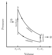
Fig. 13.11 The Otto cycle.
